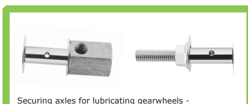
Securing axles for lubricating gearwheels - straight or right-angled
